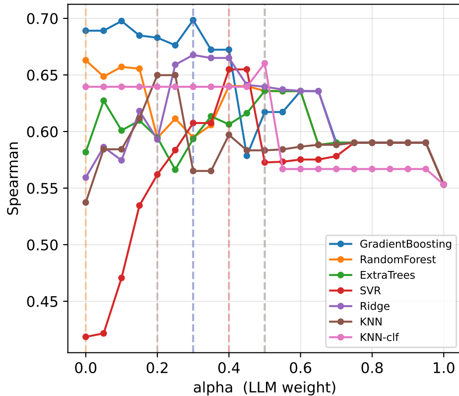
Spearman r
