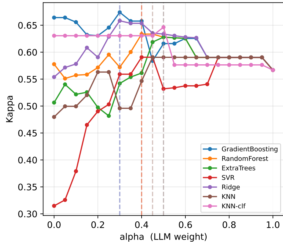
Quadratic Weighted Kappa
